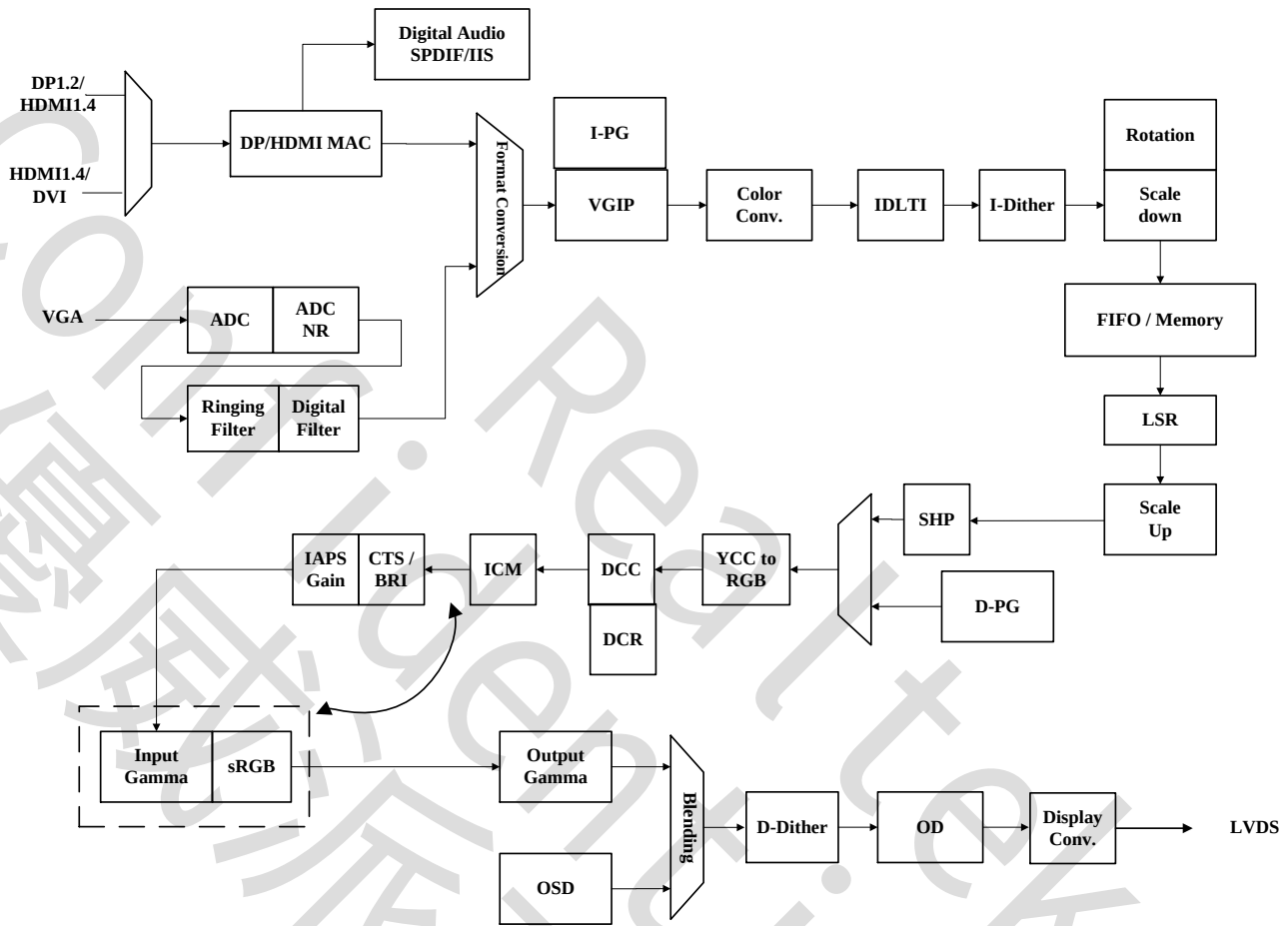
Figure 1. Block Diagram
